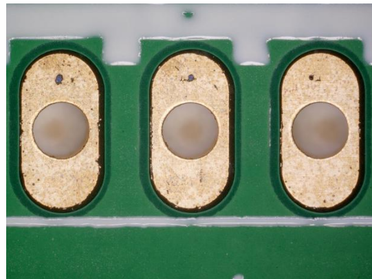
Photo(s) of sample A2210317737101001 after test(50X)
